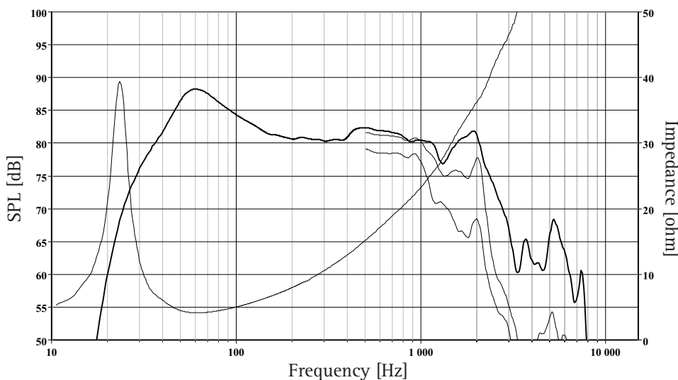
The frequency responses above show measured free field sound pressure in 0, 30, and 60 degrees angle using a 31l closed box. Input 2.83 V RMS , microphone distance 0.5m, normalized to SPL 1m. The dotted line is a calculated response in infinite baffle based on the parameters given for this specific driver. The impedance is measured in free air without baffle using a 2V sine signal.
