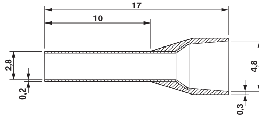
Dimensional drawing
