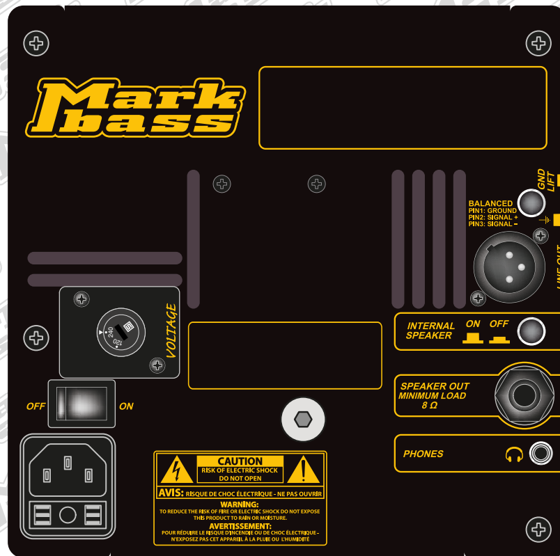
REAR PANEL
