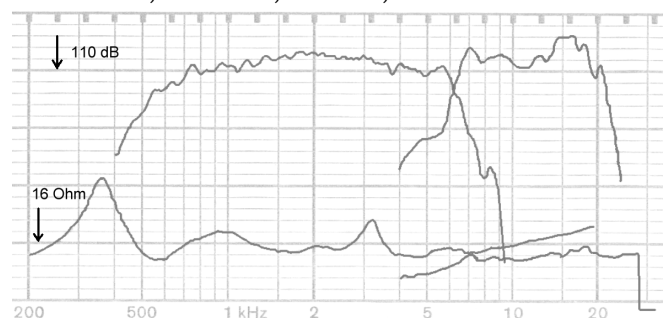
BMS 4592 ND, 2230 Horn, 1W / 1m, 4 V RMS
